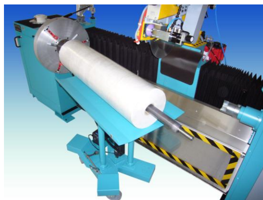
THW3S in loading position
